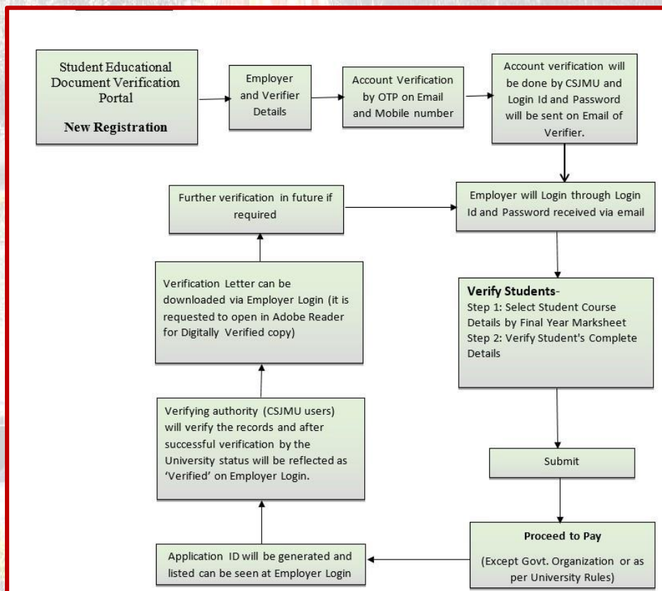
Fig. 10- Flowchart of CSJMU's faceless digital services
